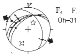
Figure 13. Brittle deformation phases reconstructed by means of the palaeostress-fields
